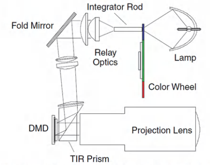
Figure 2. Generic Telecentric Optical System Components Using a TIR Prism
